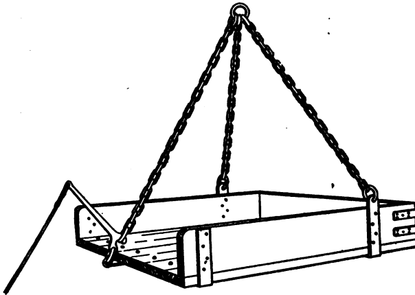
Fig. 108. Skip or Scale-pan.
